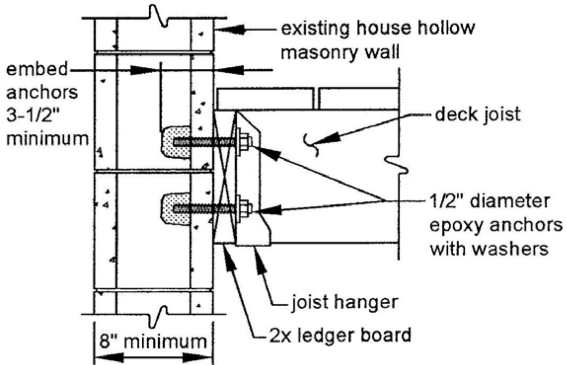
ATTACHMENT OF LEDGER BOARD-TO-FOUNDATION WALL (HOLLOW MASONRY)
